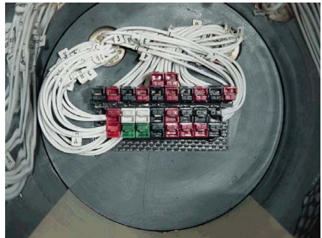
Figure 3: Through-hull electrical connections
