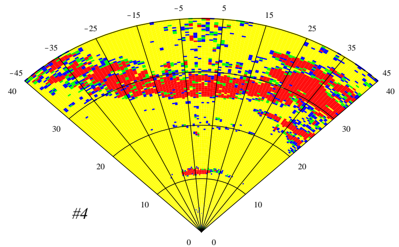
Fig. 3: A sequence of sonar images for a sample gate approximately 10 feet in front of a wall as Subjugator draws closer to the gate (red indicates a strong return, while yellow indicates no return).
