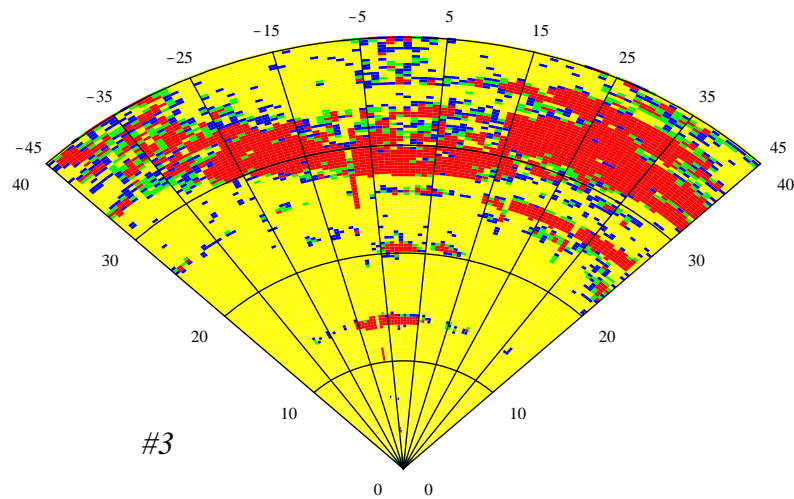
Fig. 3: A sequence of sonar images for a sample gate approximately 10 feet in front of a wall as Subjugator draws closer to the gate (red indicates a strong return, while yellow indicates no return).
