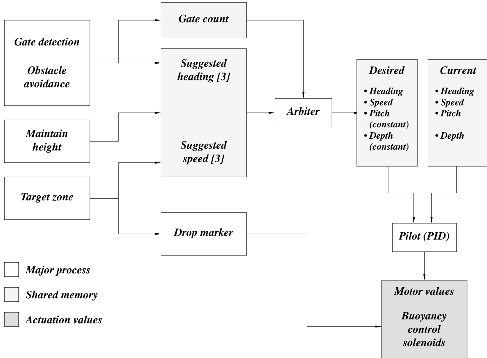
Fig. 4: Overall software architecture for SubjuGator.
